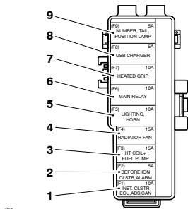
Fuse Box 1
