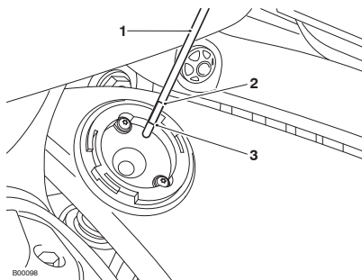
Motoröl-Peilstab
