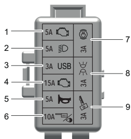
Fuse Box 2
