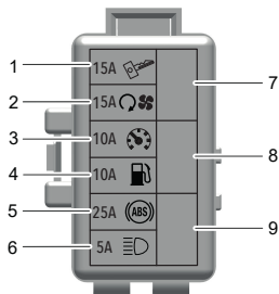
Fuse Box 1
