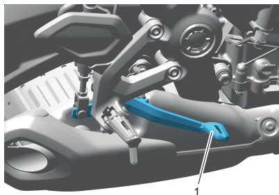
1. Rear brake pedal (Trident 660 shown)
