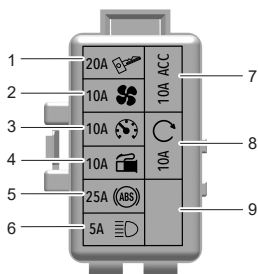
Fuse Box 1
