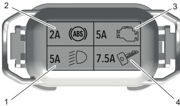
Fuse Box 2
