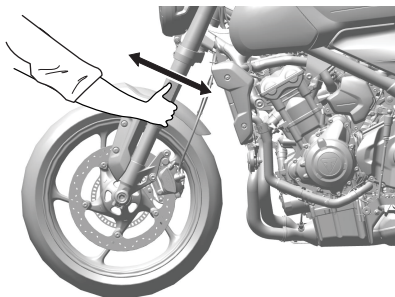
Inspecting the Steering for Free Play (Trident 660 shown)
